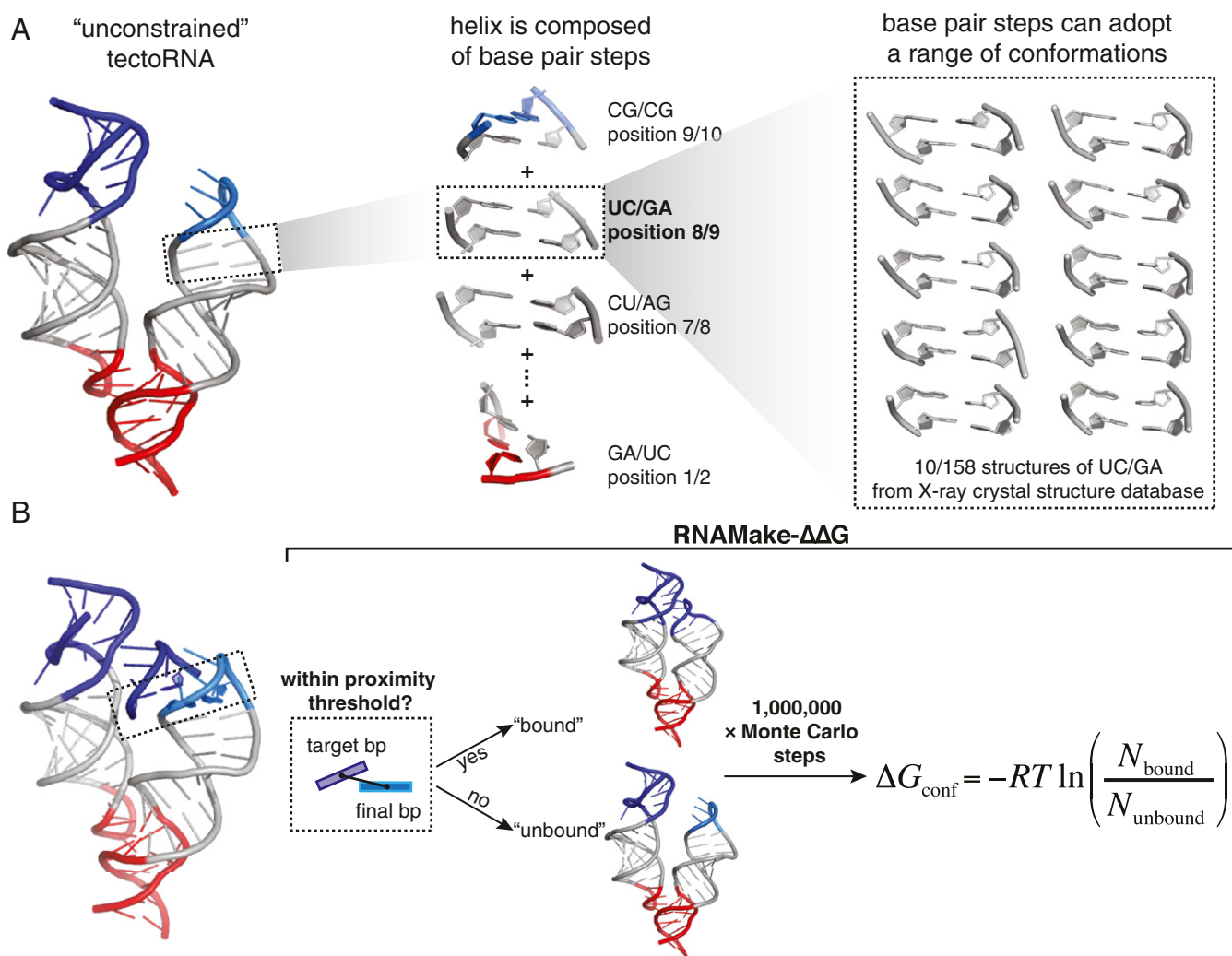
Fig. 2. Ensemble model for RNA helices allows prediction of tectoRNA assembly energetics. (A, Left) The modeled structure of the unconstrained tectoRNA (i.e., with one contact formed) is shown. The global structure was assembled from the structures of its constituent elements, including the base-pair steps that compose the helical regions. (A, Center) Example base-pair steps are shown for the chip-piece helix. Each base-pair step can adopt an ensemble of many possible conformations, which were derived from examples of that base-pair step in the crystallographic database. (A, Right) Example conformations within the UC/GA conformational ensemble are shown. (B) Starting with the unconstrained tectoRNA as shown in A, a Monte Carlo simulation was performed. At each step of the simulation, the structure of one base-pair step in the tectoRNA was replaced with a new state from its conformational ensemble. The new structure of the unconstrained tectoRNA assembly was evaluated for whether it was “bound” or “unbound,” according to the translational and rotational distances from the target base pair to the final base pair. One million steps were performed, and the total number of computed bound and unbound tectoRNA conformations were used to calculate the free energy change between the bound and the unbound tectoRNAs ( \Delta G_{\text{conf}} ).
