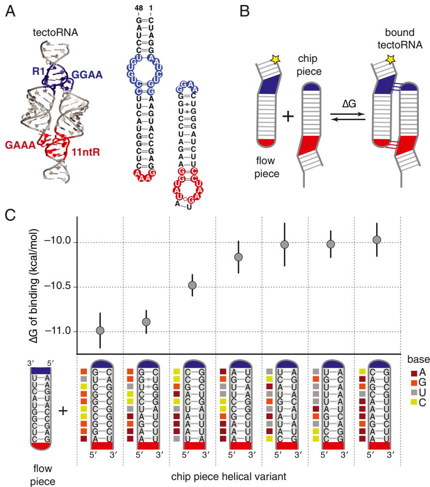
Fig. 1. Free energy of tectoRNA binding depends on helix sequence. (A) Structure of tectoRNA homodimer [Protein Data Bank (PDB): 2ADT] with 2 tertiary contacts (GAAA-11nt). One of these tertiary contacts is replaced (GGAA-R1; blue) to convert the complex to the heterodimer used in this study (32). On the right is the sequence and secondary structure of the wild-type tectoRNA interaction. Numbers indicate the “position” within the chip-piece helix. (B) In our experimental setup, one piece of the heterodimer was fluorescently labeled and free in solution (the “flow piece”), while the other was immobilized on the surface of a sequencing chip (chip piece). Quantification of the bound flow piece to the chip surface allowed determination of the free energy of binding ( \Delta G ) to form the bound tectoRNA. (C) Free energy of binding of the flow piece to 7 distinct chip-piece variants. Error bars are 95% CI on the measured \Delta G . The sequence of the flow- and chip-piece helices is indicated (Bottom).
